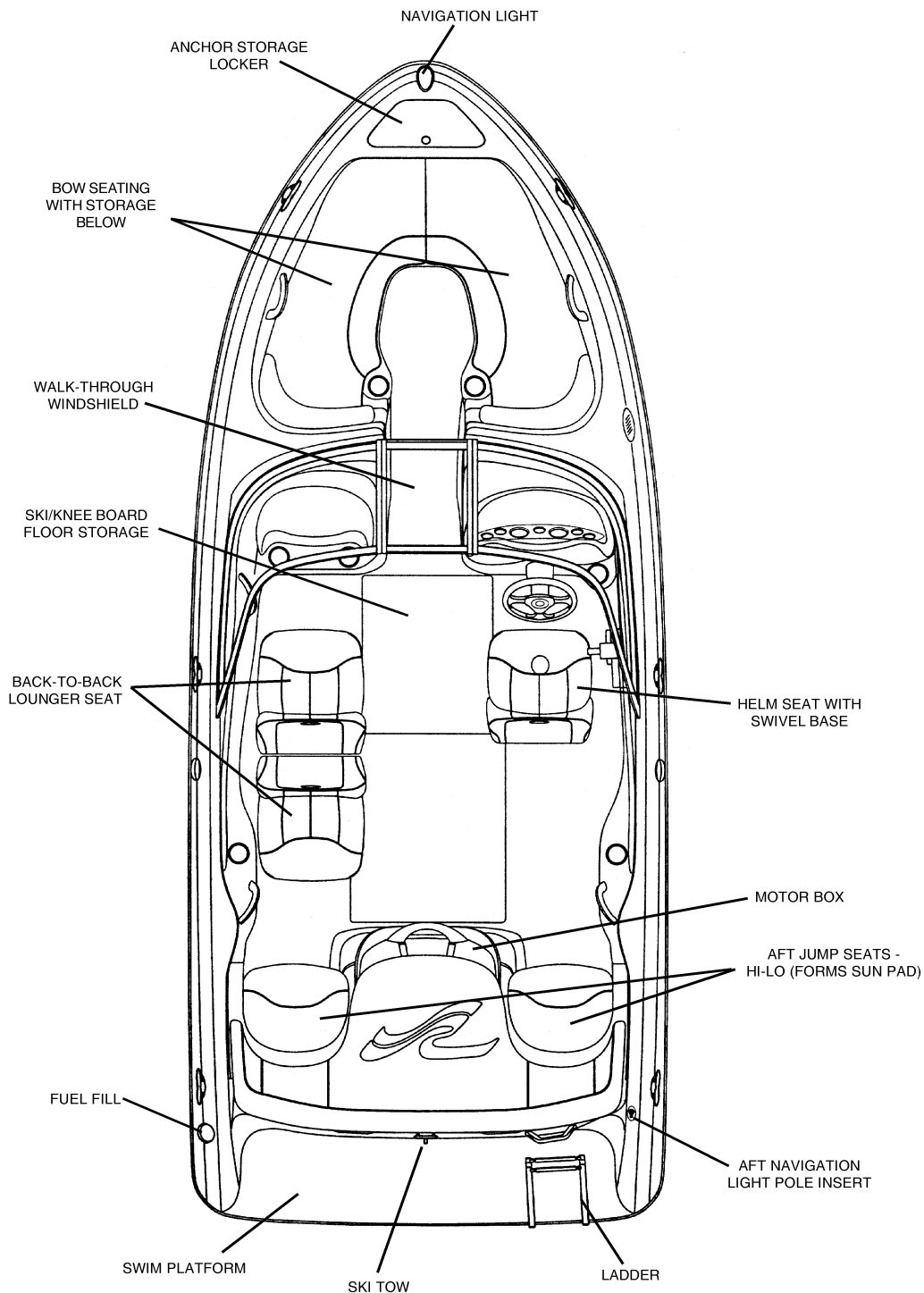
GENERAL LAYOUT (OPTION) (FIG. 2.5.1)
