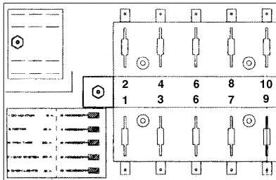
ACCESSORY FUSE BLOCK (LOCATED BEHIND DASH ACCESS PANEL) (FIG. 6.4.2)
