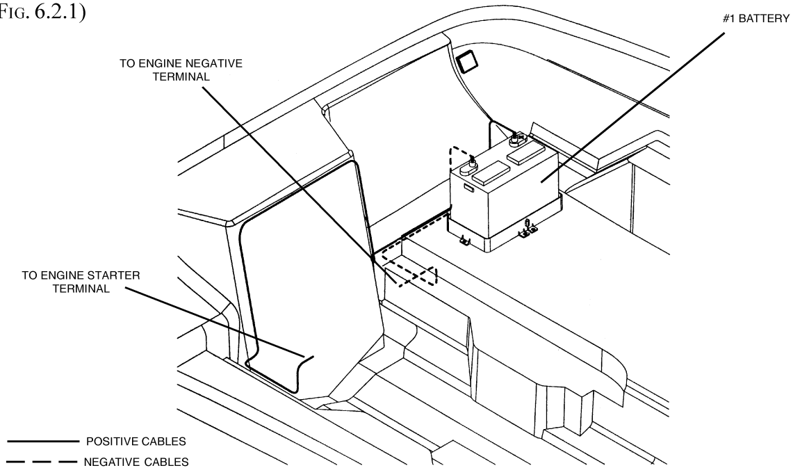
BATTERY CABLE ROUTING WITH BATTERY SWITCH OPTION (FIG. 6.2.2)
