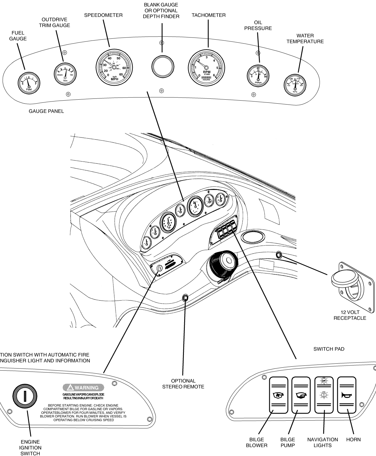
HELM GAUGES AND SWITCHES (FIG. 2.7.1)
