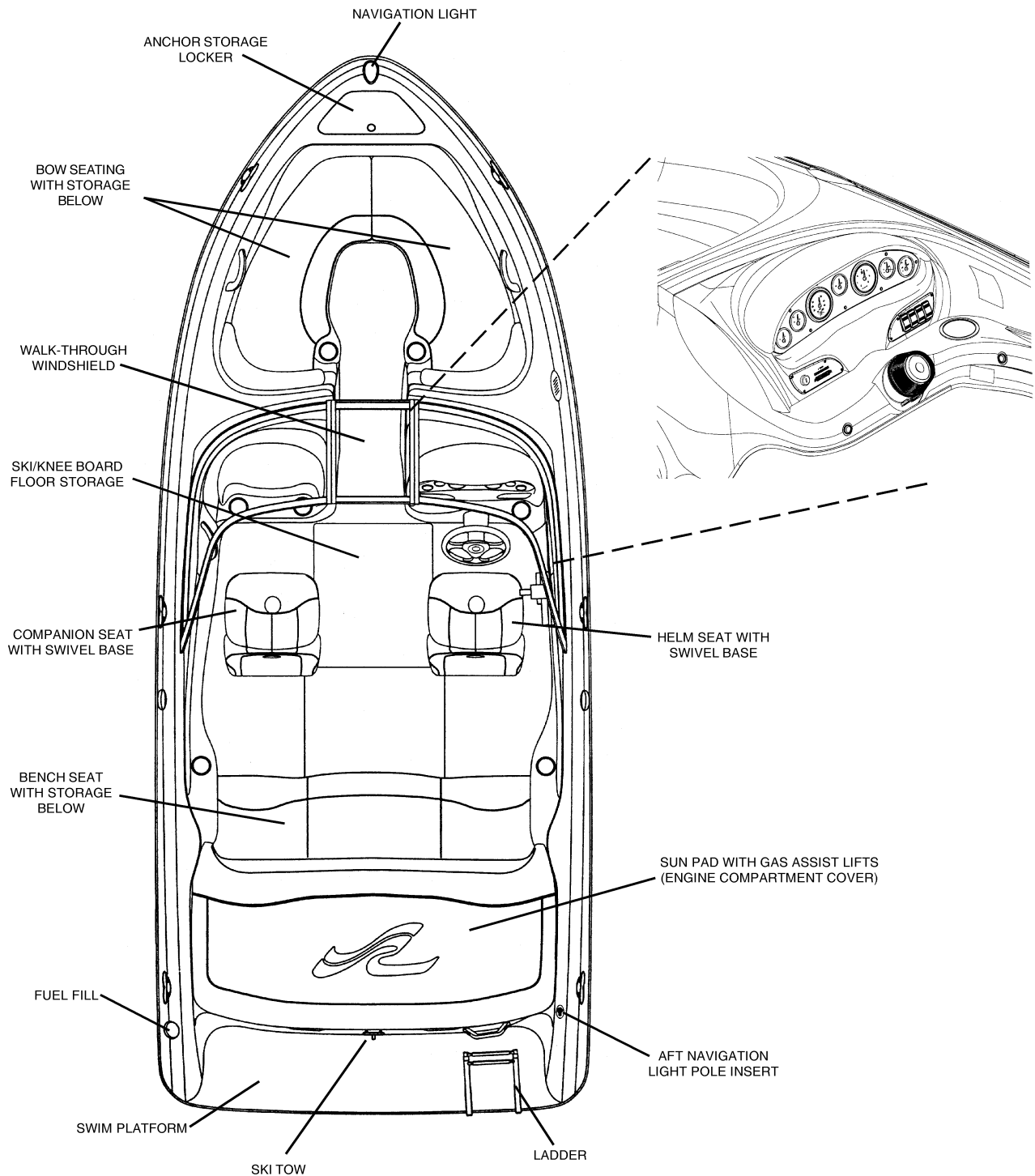
GENERAL LAYOUT (STANDARD) (FIG. 2.4.1)
