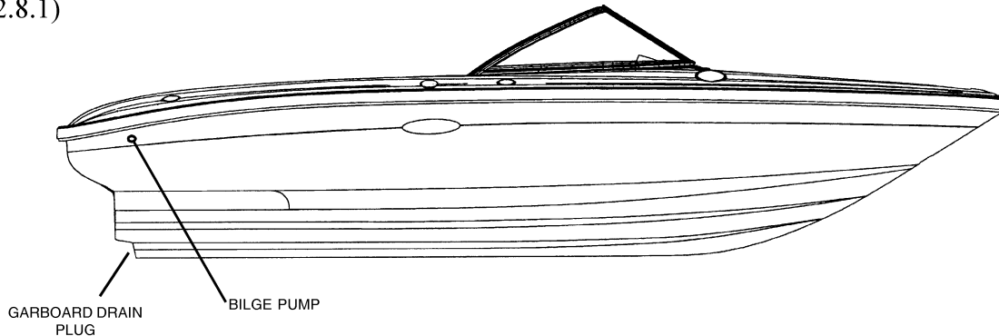
STARBOARD THROUGH-HULL CUTOUTS (FIG. 2.8.1)
