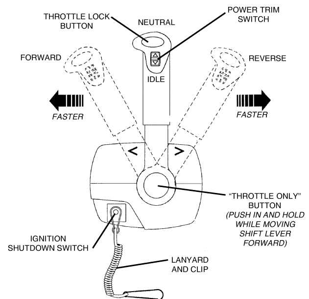
GEAR SHIFT AND THROTTLE CONTROL (FIG. 2.8.2)
