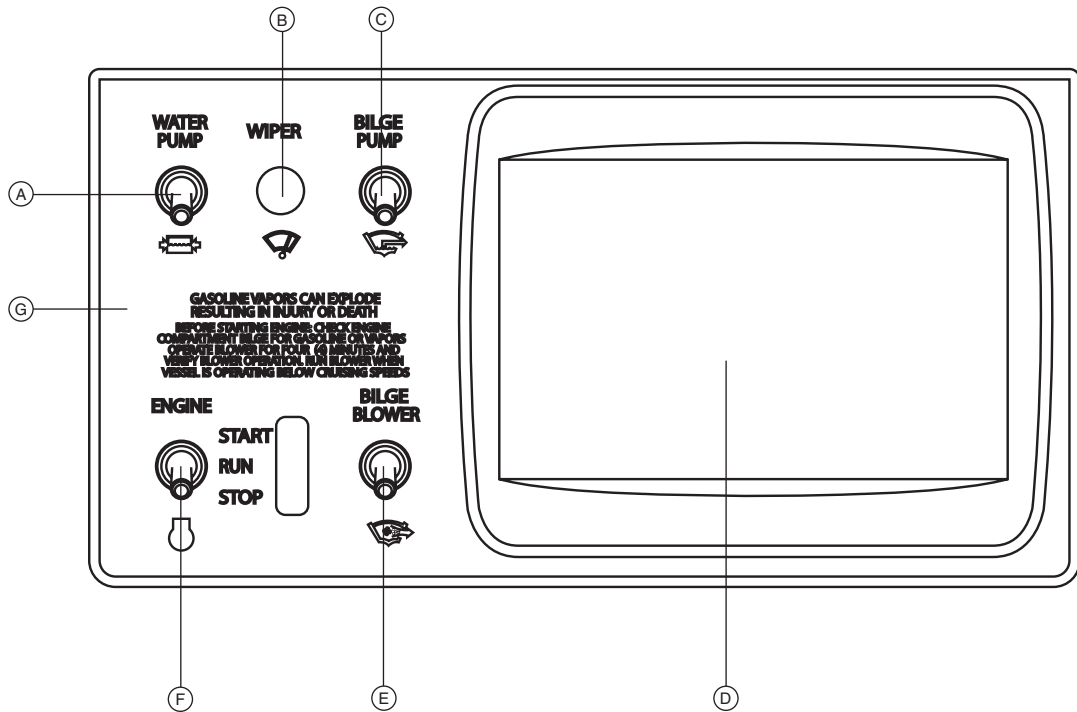
SWITCH PANEL, STARBOARD (FIG. 11.1)
