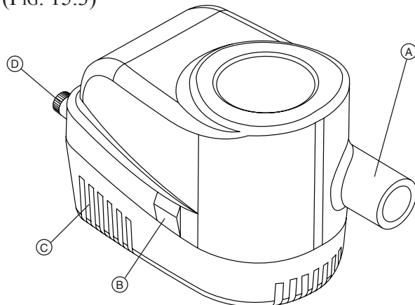
TYPICAL BILGE PUMP AND FLOAT SWITCH (FIG. 15.3)
