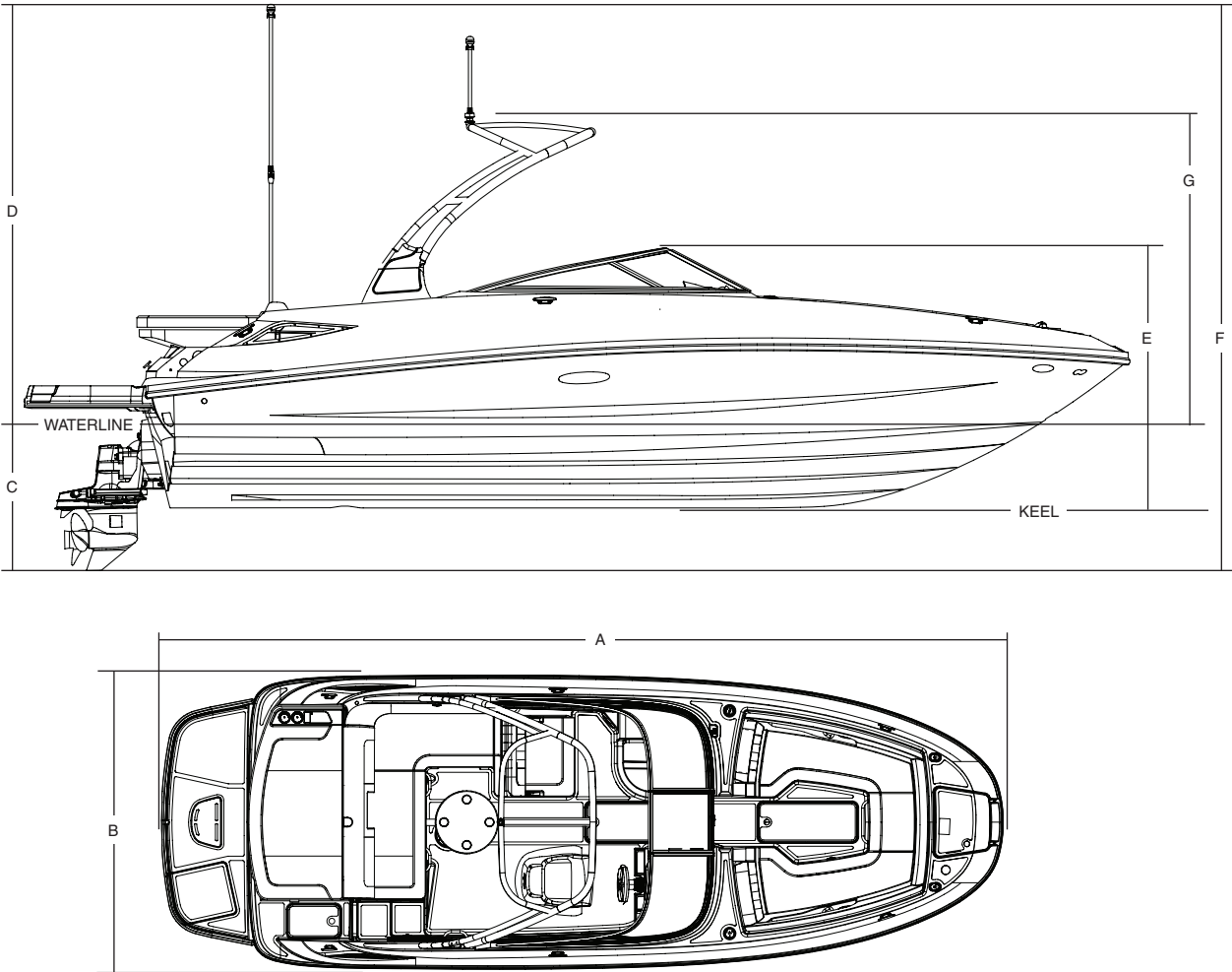
BOAT DIMENSIONS AND CLEARANCES (FIG. 8.1)
