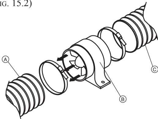
TYPICAL BILGE BLOWER (FIG. 15.2)
