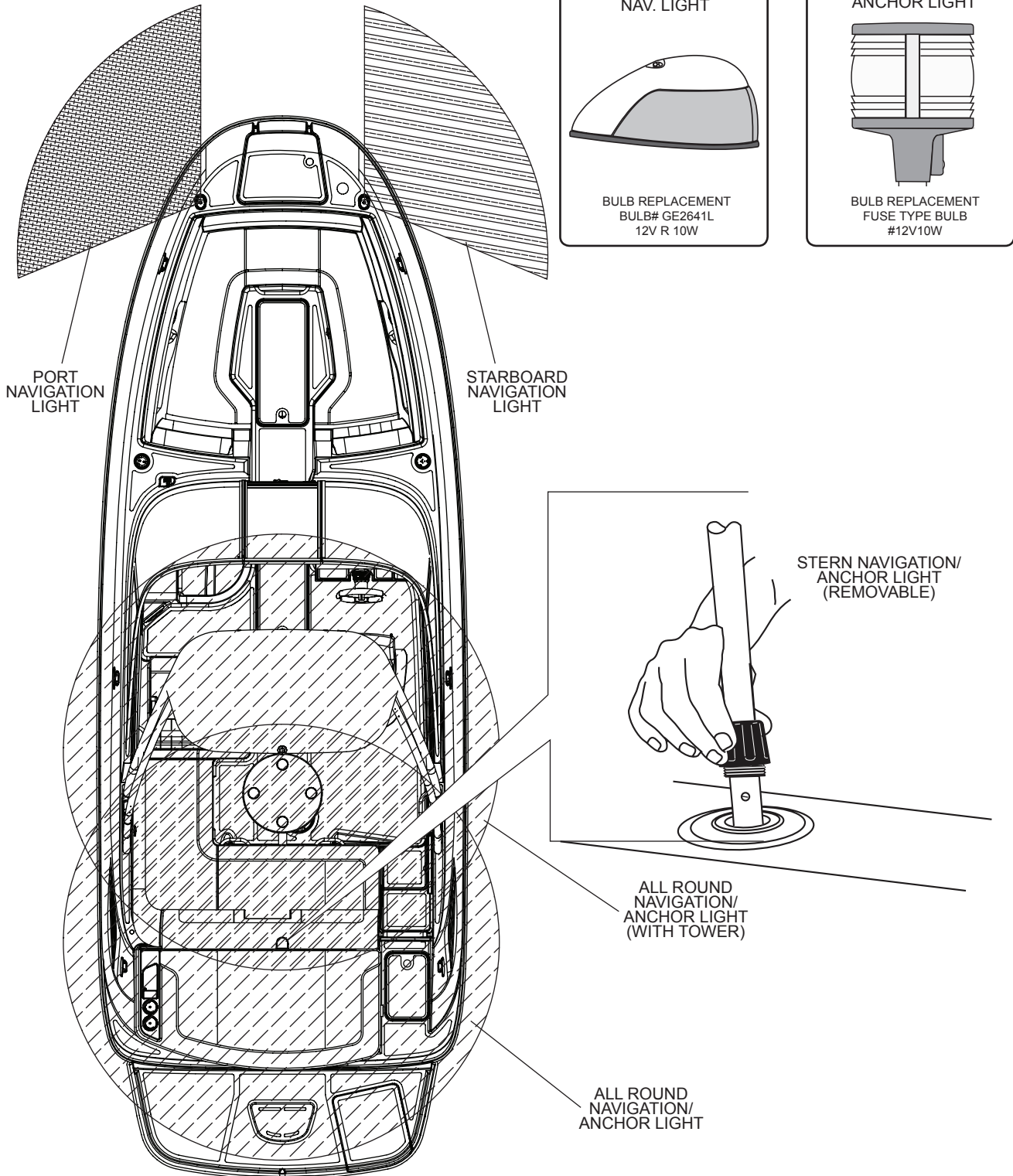
NAVIGATION AND ANCHOR LIGHTS (FIG. 14.1)
