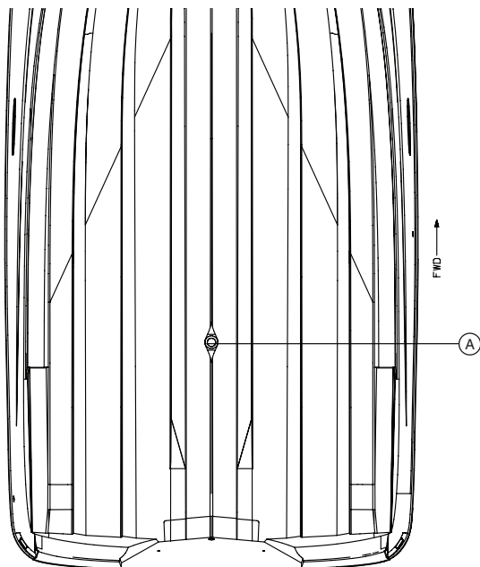
BILGE AND TRANSOM THROUGH-HULL CUTOUTS (FIG. 9.3)
